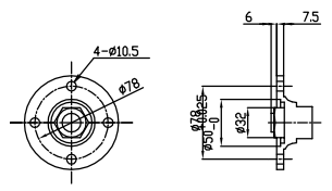
DETAIL OF COUPLING SCALE 1:3
